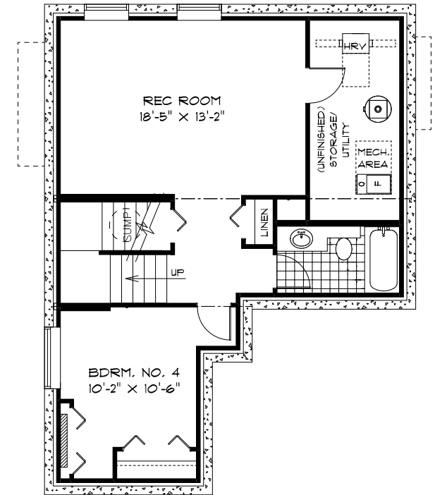
OPTIONAL LOWER LEVEL FLOOR PLAN
