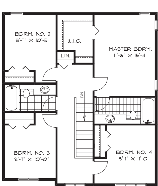
BROADVIEW - DG 21 SECOND FLOOR PLAN ( 963 SQ. FT. )
