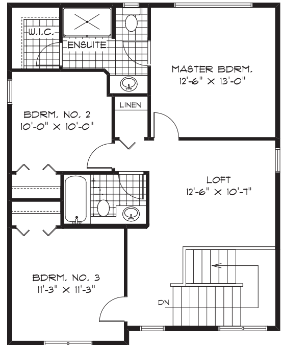
20 ATLAS SECOND FLOOR PLAN ( 925 SQ. FT. )
