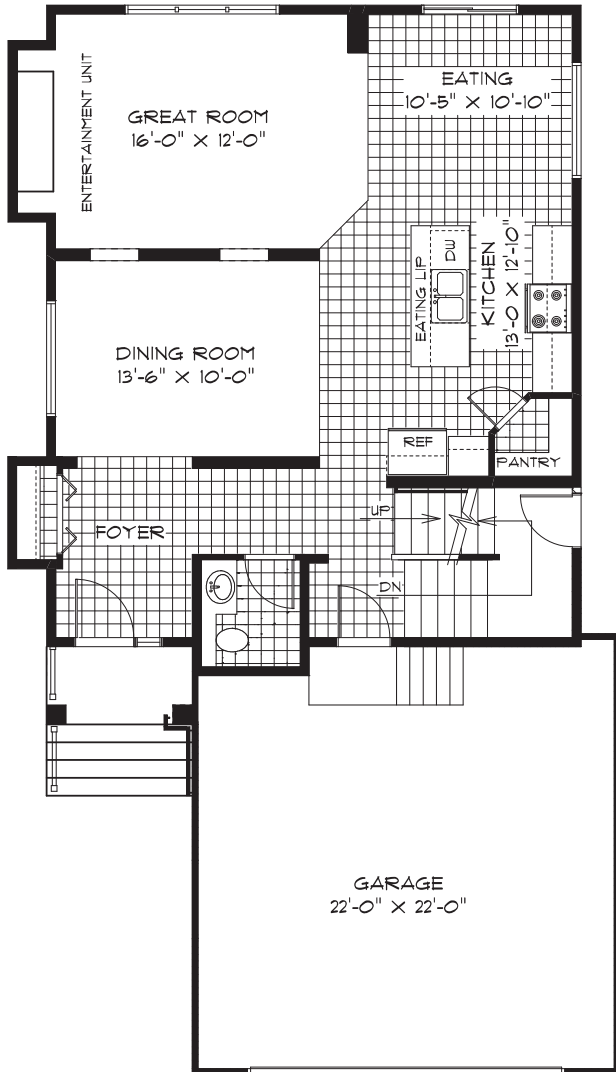
20 ATLAS MAIN FLOOR PLAN ( 928 SQ. FT. )
