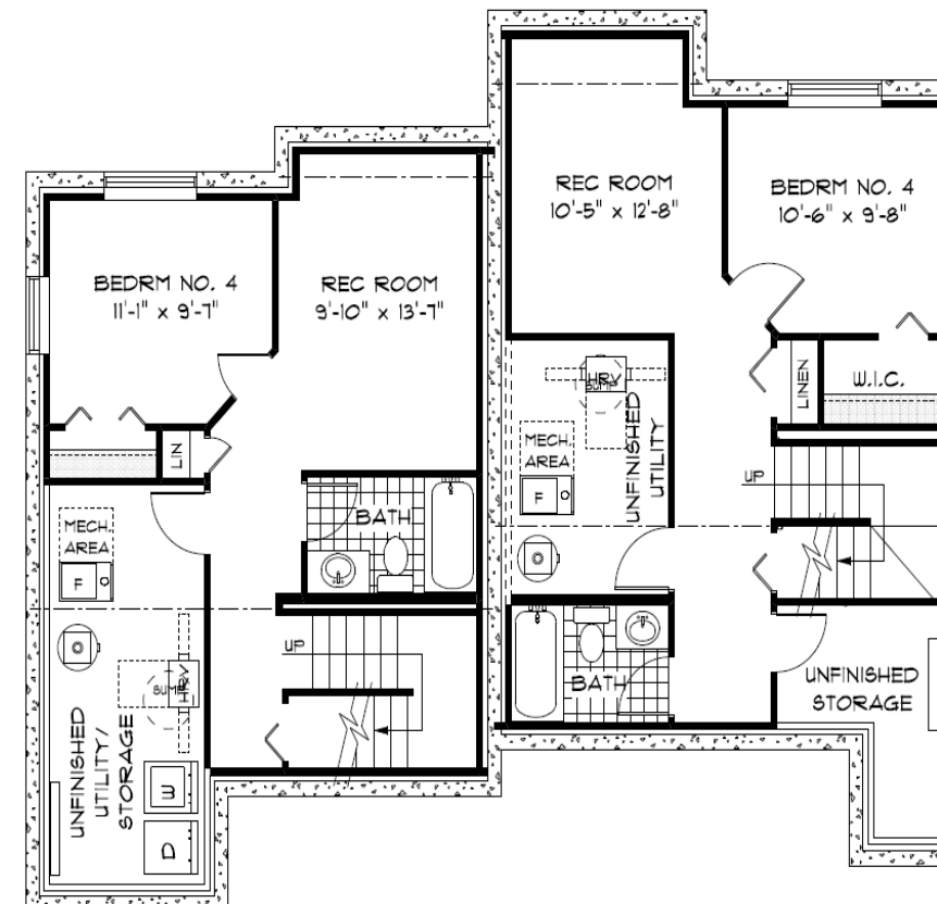
OPTIONAL LOWER LEVEL FLOOR PLAN UNIT 1 | UNIT 2 Finished Area: 443 Sq. Ft. | Finished Area: 413 Sq. Ft.
