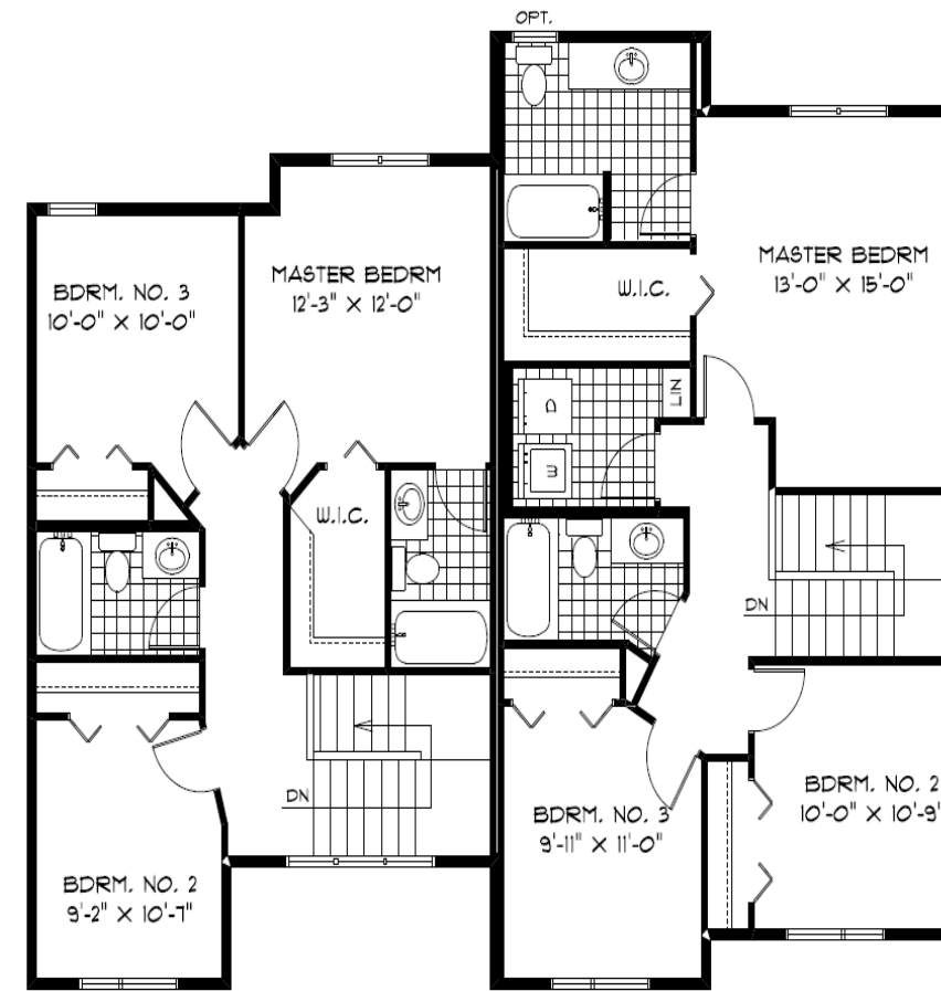
SECOND FLOOR PLAN UNIT 1 | UNIT 2 854 Sq. Ft. | 707 Sq. Ft.
