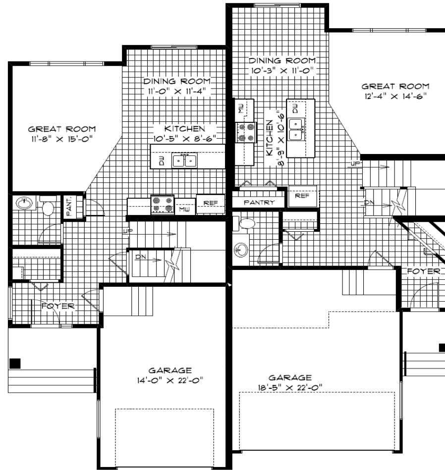
MAIN FLOOR PLAN UNIT 1 | UNIT 2 707 Sq. Ft. | 742 Sq. Ft.
