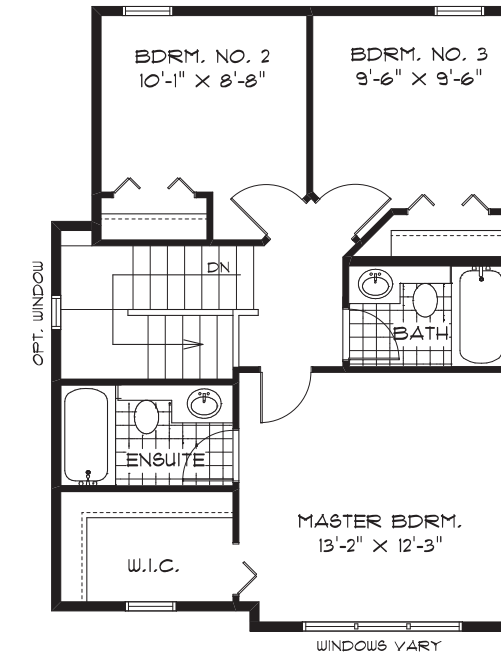
SECOND FLOOR PLAN (682 SQ. FT.)
