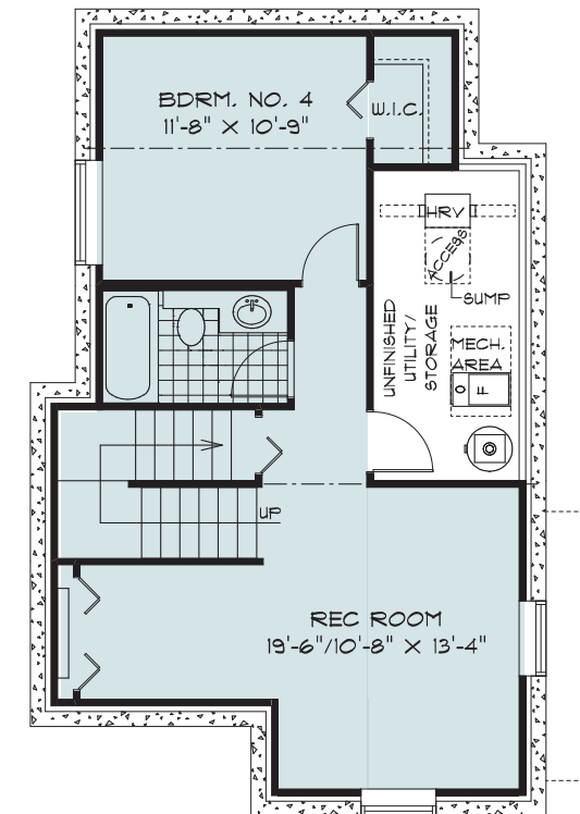
OPTIONAL LOWER LEVEL FLOOR PLAN (FINISHED AREA 504 SQ. FT.)
