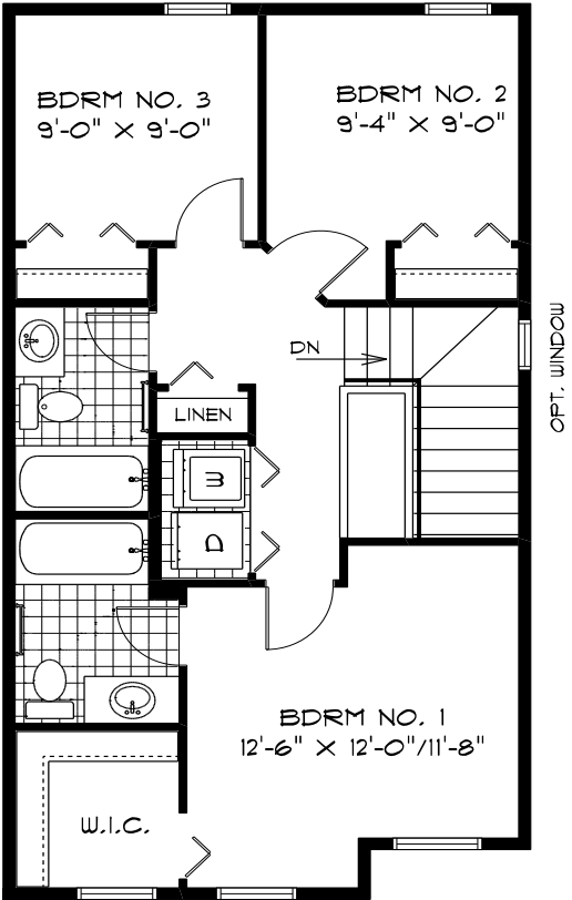
SECOND FLOOR PLAN 699 Sq. Ft.
