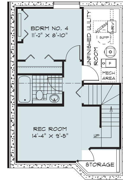
OPTIONAL LOWER LEVEL FLOOR PLAN ( FINISHED AREA 373 SQ. FT. )
