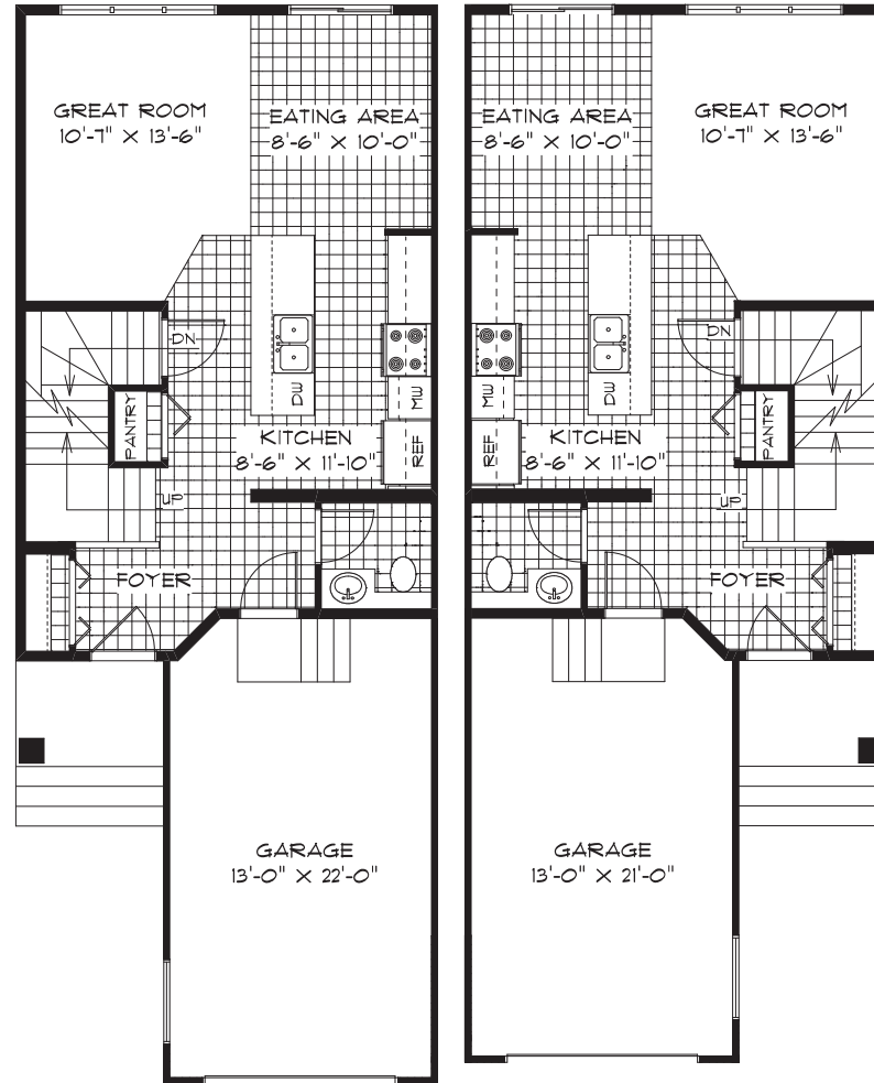
SG8 - UNIT 1 MAIN FLOOR PLAN ( 596 SQ FT )
