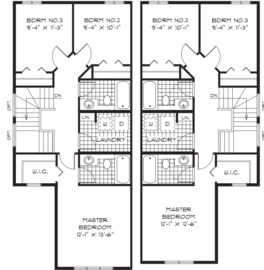
SG8 - UNIT 2 SECOND FLOOR PLAN ( 787 SQ FT )
