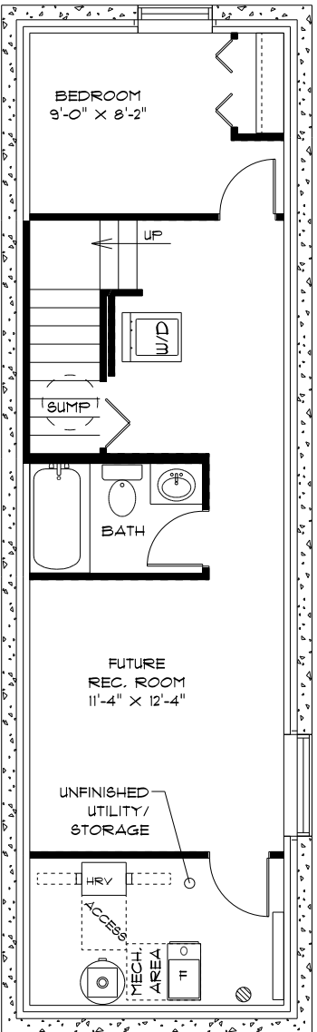
OPTIONAL LOWER LEVEL FLOOR PLAN Finished Area: 386 Sq. Ft.
