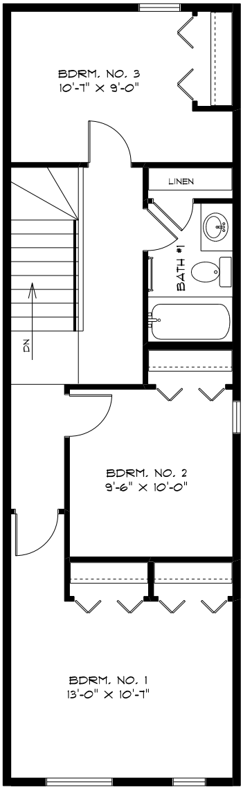
SECOND FLOOR PLAN 3 BEDROOM OPTION 658 Sq. Ft.
